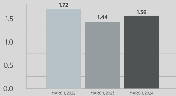
Current Ratio
