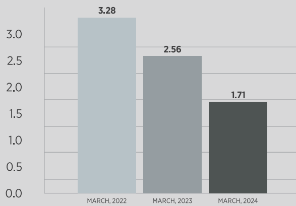
Debt-Equity Ratio
